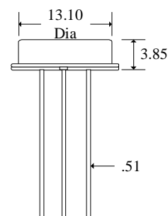
HC-37/U LOW PROFILE
